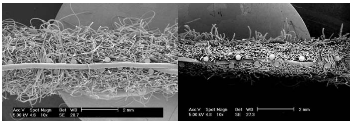
Figure 3. Untested sample (on the left) and tested sample (on the right)
