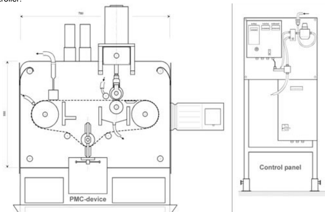
Figure 2. The principal picture of the test device is on the left. The dashed line represents the endless felt sample in the machine direction. The control panel for the device and the IR-controller are on the right
