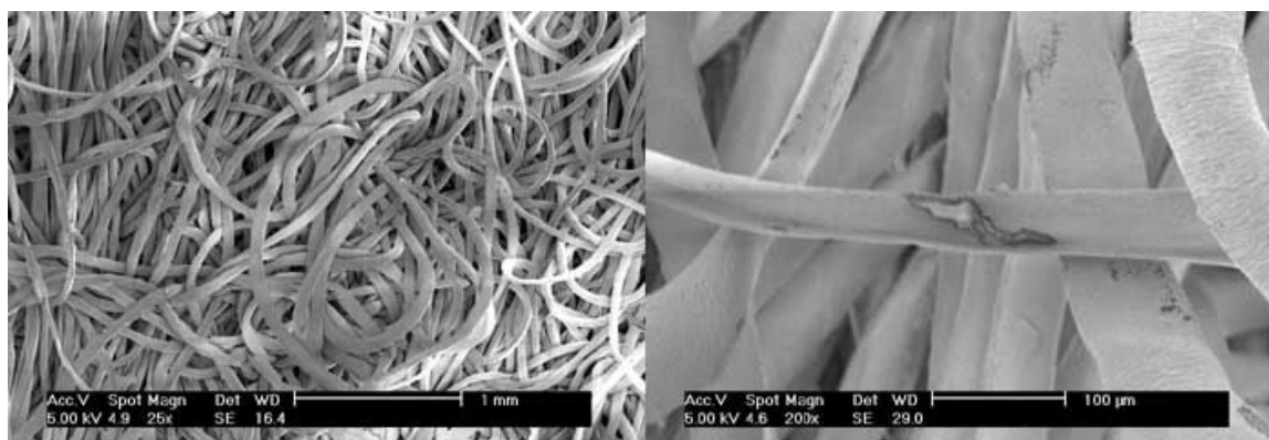
Figure 4. Surface of tested sample (on the left) and some flat staple fibres (on the right) on the paper side of the felt
