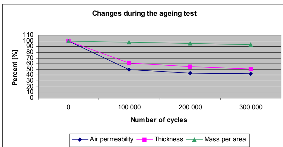
Figure 5. Changes in properties of the felt sample during the ageing test
