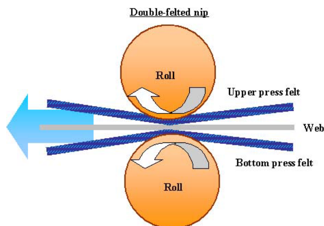
Figure 1. This nip builds up about two rolls and two press felts. Between them the water is removed from paper web
